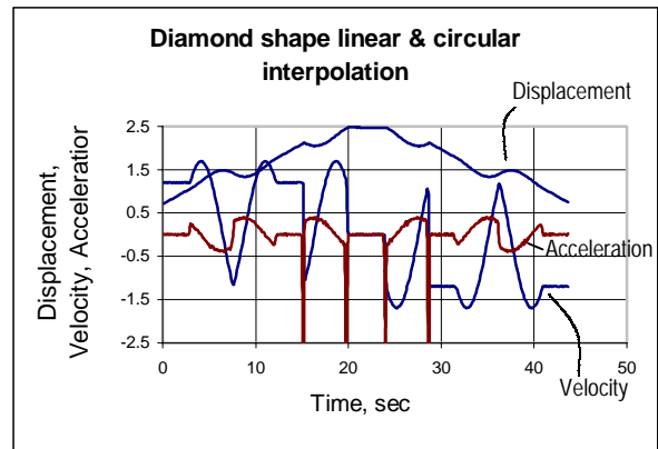
Fig. 5 A diamond (shown in Fig. 4) tool path, velocity and acceleration measured in the x-direction. The feed rate was 10 in/min. The top trace is the displacement(in), the middle trace is the velocity(in/sec) and the bottom trace is the acceleration(in/sec 2 )
