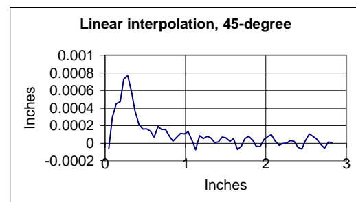
Fig. 2 A measurement lateral deviation of a linear interpolation inclined 45 degree from x-axis.
