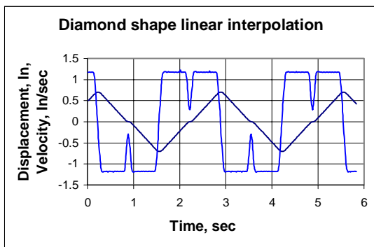
Fig. 3 A diamond shape tool path and its velocity measurement in the x-direction, The velocity dropped to 25% at the corners.
