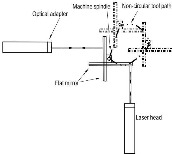
Fig. 1 A typical laser setup for the Non-circular contouring measurement.
