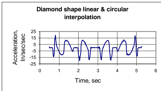
Fig. 6b Same as in Fig. 5, except the feed rate was 100 in/min. The trace is the acceleration (in/sec 2 ).
