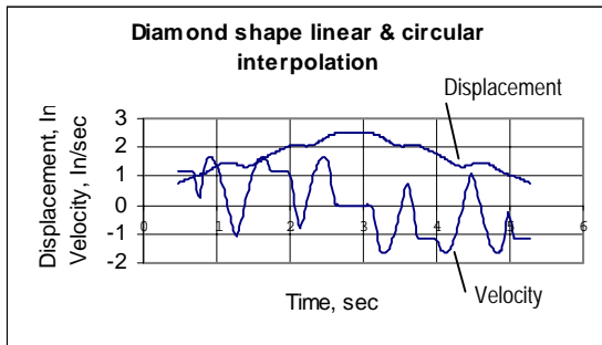
Fig. 6a Same as in Fig. 5, except the feed rate was 100 in/min. The top trace is the displacement (in) and the middle trace is the velocity (in/sec).
