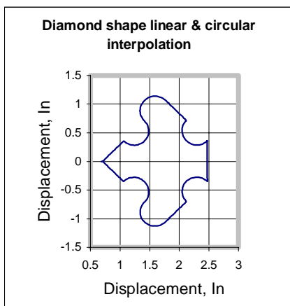
Fig. 4 A diamond shape tool path with half-circles, 45 degree and 135 degrees lines, a vertical and horizontal lines.
